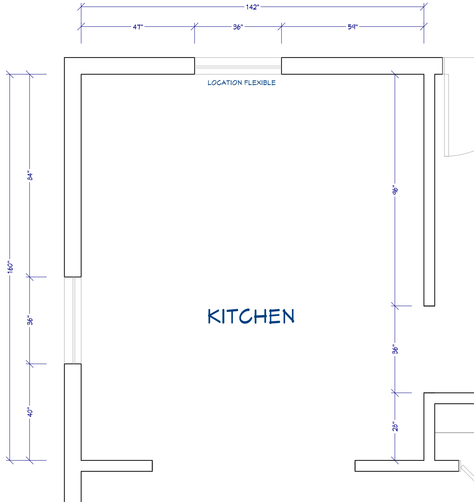
KITCHEN PLAN
