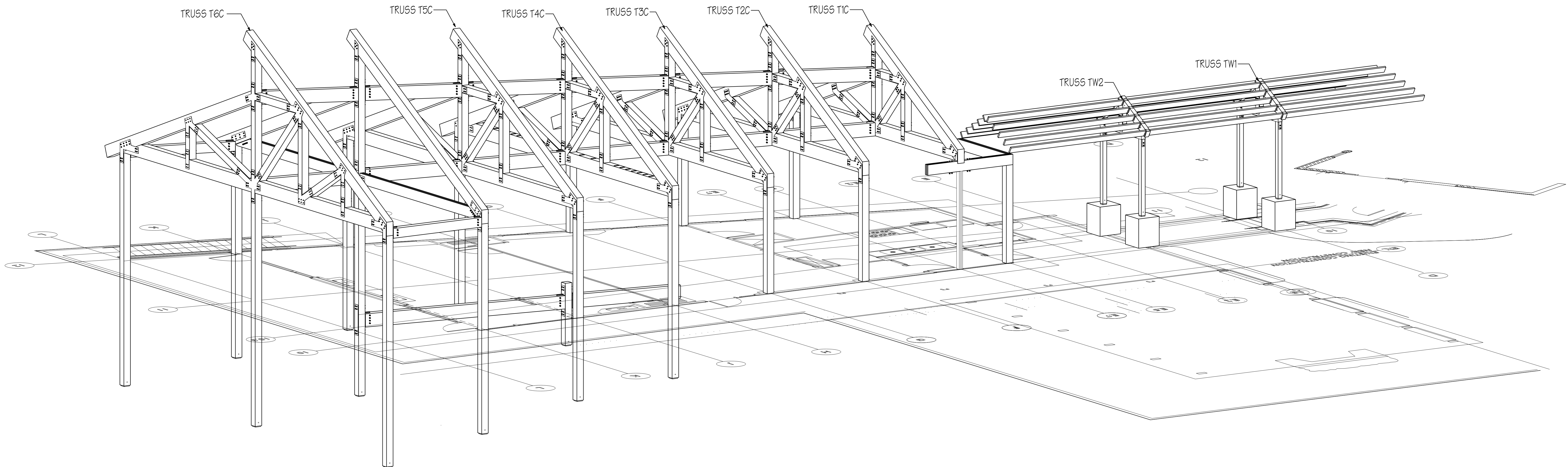
3D REAR LEFT PERSPECTIVE OF CLASSROOM BUILDING AND BREEZEWAY
